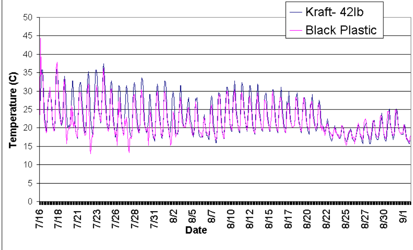
Figure 6: Kraft-42 paper (plastic-coated) and Black Plastic
