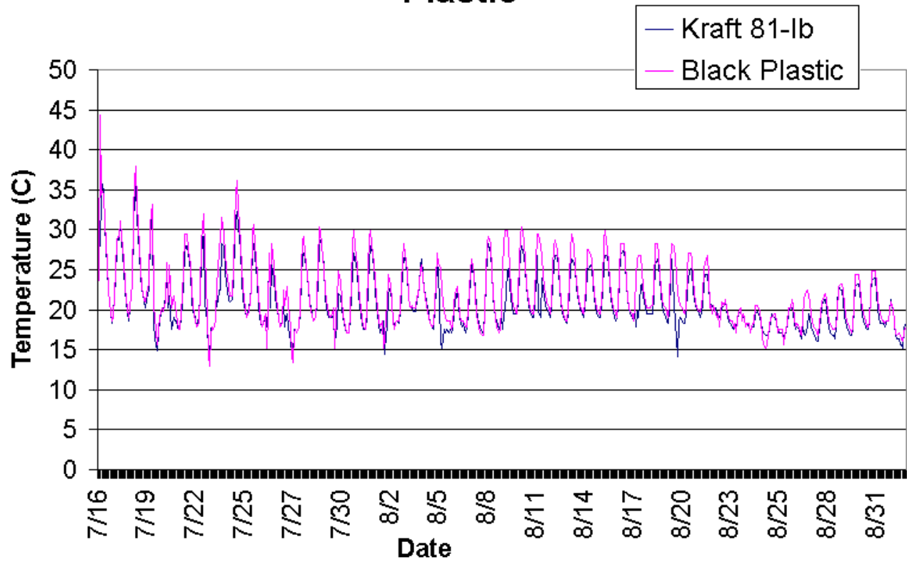
Figure 5: Garden Bio-Film and Black Plastic
